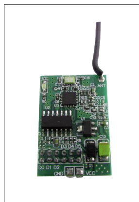
RF-sender 10700115
